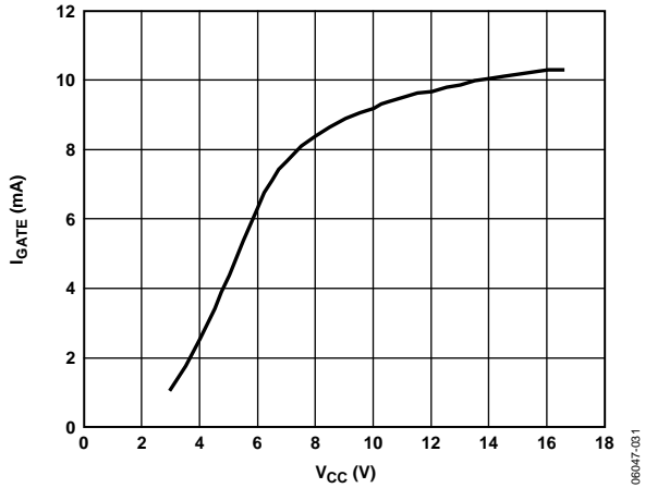
Figure 10. Gate Pull-Down Current vs. Supply Voltage at V_{GATE} = 5V
